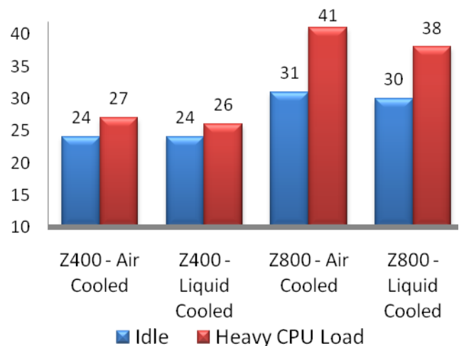
Figure 1 - Acoustic comparison between air and liquid cooled systems
