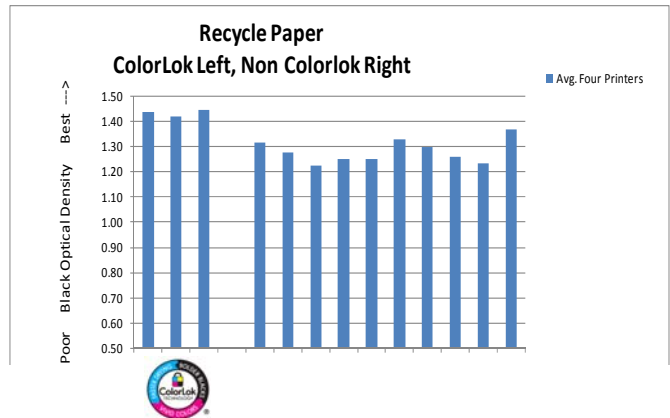
Figure 2. Improvement from ColorLok(R) treatment for optical density
