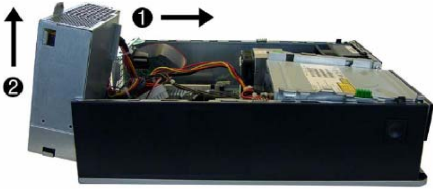
FIGURE 8: Power supply cover screw locations (top)
