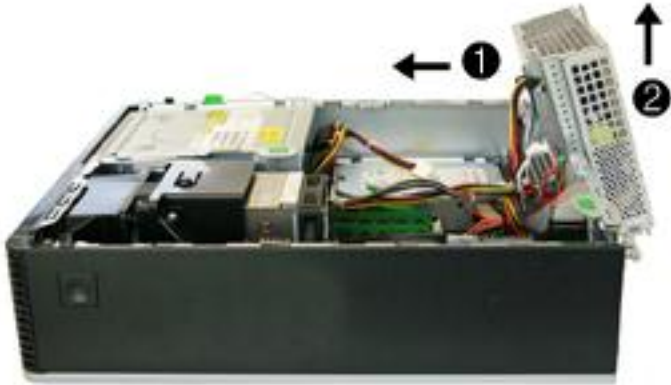
FIGURE 8: Power supply cover screw locations (top)
