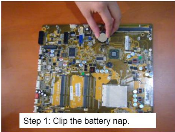
Figure 3 : Remove Battery from MB.
