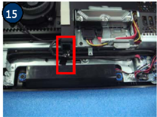
15 Tear cable routing tape for cable shielding L and put out those cables form cable shielding.
