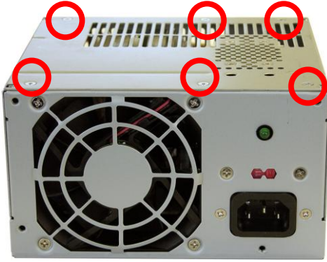
FIGURE 16: POWER SUPPLY 3: Screw locations
