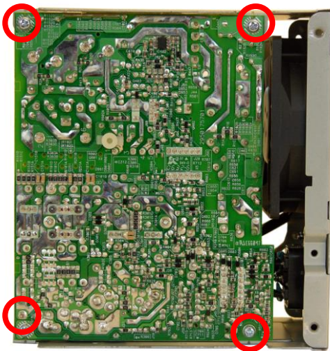
FIGURE 11: POWER SUPPLY 1: Large PCA screw locations
