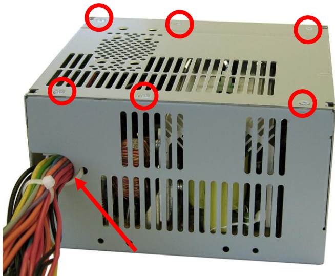
FIGURE 26: POWER SUPPLY 6: Screw and plastic tie locations
