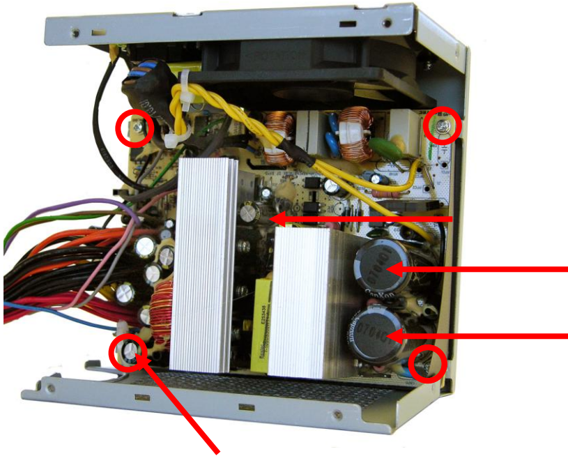
FIGURE 26: POWER SUPPLY 6: Screw and plastic tie locations
