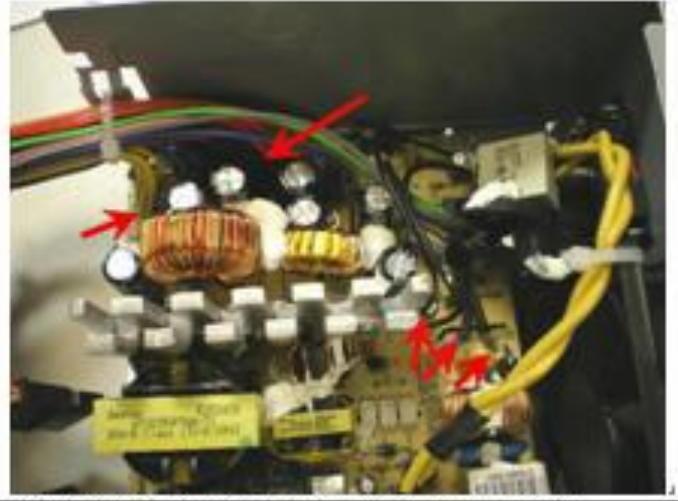
Figure 16 : Heat the solder of Electrolytic Capacitors.
