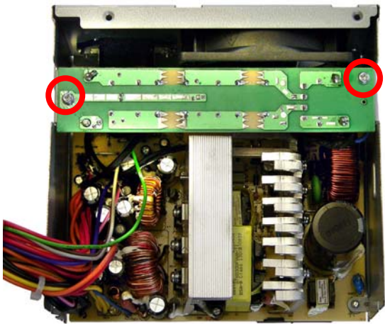
FIGURE 12: POWER SUPPLY: Large PCA screws to remove
