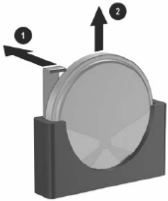
FIGURE 10: Type 3 battery holder
