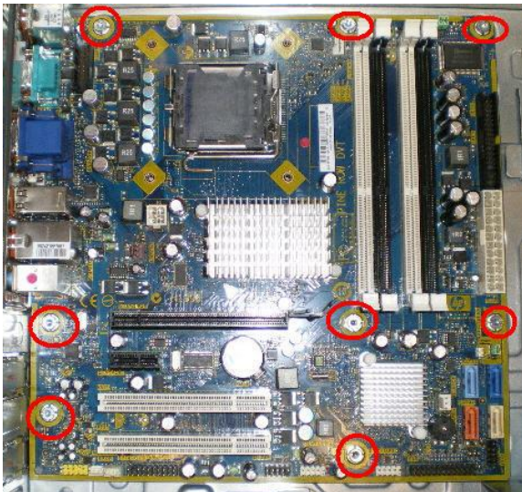
Figure 5: Remove the system board
