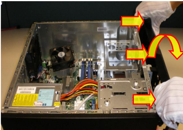
Figure 3: Remove the front bezel
